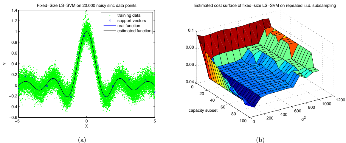
Figure 3.15: Illustration of fixed size LS-SVM on a noisy sinc function with 20,000 data points: (a) fixed size LS-SVM selects a subset of the data after Nyström approximation. The regularization parameter for the regression in the primal space is optimized here using the Bayesian framework; (b) Estimated cost surface of the fixed size LS-SVM based on random subsamples of the data, of different subset capacities and kernel parameters.
