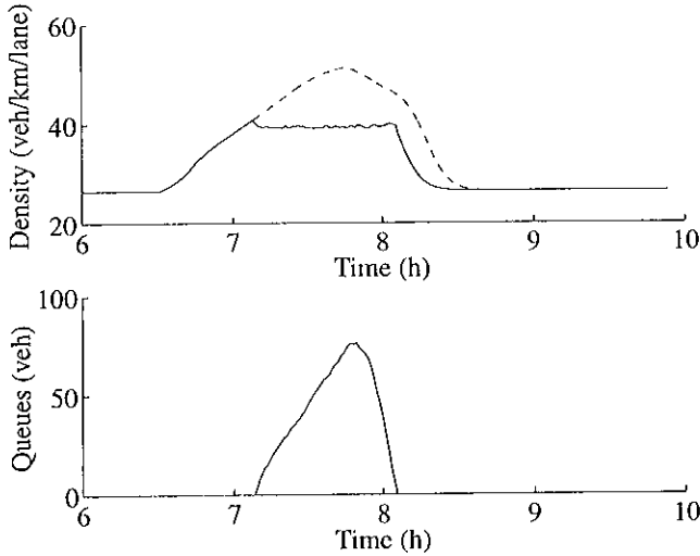
Fig. 5. Plot of the evolution of the density in the section fed by the fourth on-ramp and the queue at the first on-ramp for two model predictive control based ramp metering controllers. The solid line represents the controller using the correct model parameters ( \beta_{\text{ref}} ). The dashed line represents the controller using the perturbed parameter set ( \beta_{\text{pert}} ).
