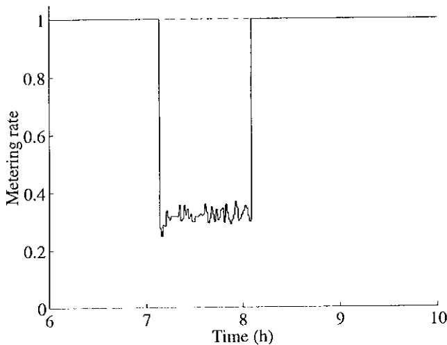
Fig. 6. Plot of the evolution of the metering rate as presented by both controllers. The solid line represents the controller using the correct model parameters ( \beta_{\text{ref}} ). The dashed line represents the controller using the perturbed parameter set ( \beta_{\text{pert}} ). Note that the controller with the perturbed parameter set never becomes active.
