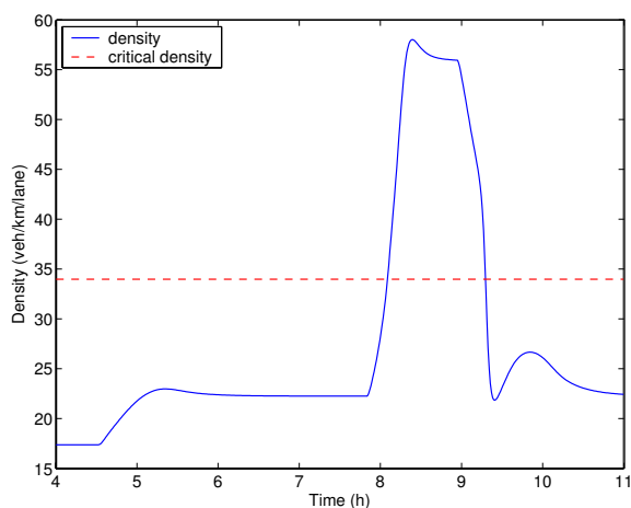
(c) Density on segment downstream of the on-ramp
