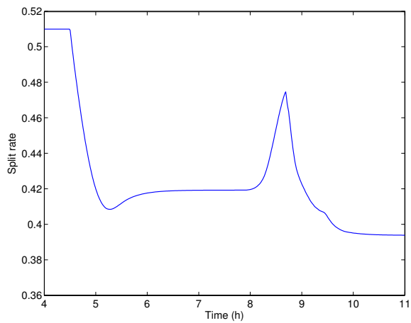
(b) Split rate toward route 2
