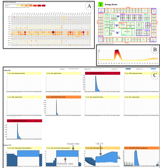
Fig. 2. Detail of Building Anomalies Detections Interface (BADI). A): Heatmap for building dataset represented per day and zone. Each square is encoded by size and color. Size: mean of the number of SDs of all variables; Color: highest SD of the variable in a specific zone. B) Line-chart showing the time in the X-axis, and the mean value of the number of SDs in the Y-axis. C) Comparative line-charts for individual variables. Each one represents the mean of the variables and the actual values. Dark-blue is for values lower than the reference value; light-blue for values greater than the reference value.
