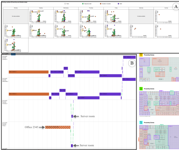
Fig. 1. Detail of Proximity Anomalies Detections Interface (PADI). A) Scatterplot matrix for all the days available. Each circle represents an employee in a specific day. B) List of timelines of the movements of a selected employee.
